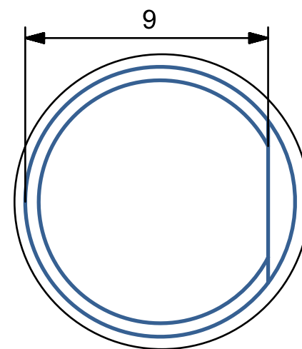
D-type shaft dimensions Scale 5:1
