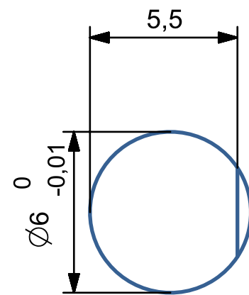
D-type shaft dimensions Scale 5:1
